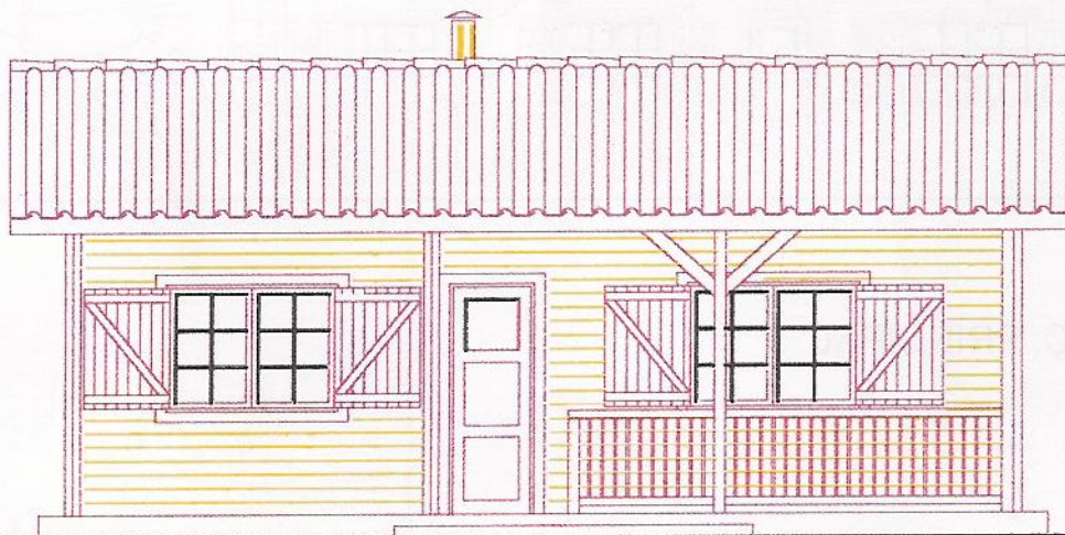
ALÇ. PRINCIPAL
